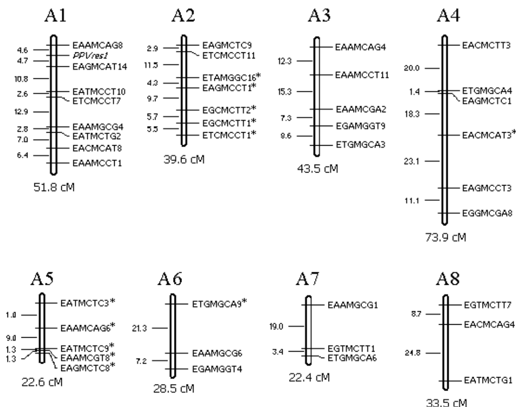
1. Partial genetic linkage map of apricot derived from the population (Stark Early Orange × Vestar) × Vestar. The phenotypic trait (PPV resistance) and the AFLP markers are indicated on the right and genetic distance in centimorgans is indicated on the left. Nineteen markers (EAAMCAG6, EAAMCCT2, EACMCCC2, EACMCCC7, EACMCTT2, EAGMCAT4, EAGMCAT5, EAGMCAT6, EAGMCAT7, EAGMCAT11, EAGMCCT8, EAGMCTC7, EATMCCT8, EATMCTC2, EGAMGGT5, EGGMCGA7, EGGMCGA10, ETAMGGC3, ETGMGCA5) remain independent. Asterisks (*) indicate distorted segregations of markers ( \chi^2 test, P < 0.05 ). Vertical lines represent linkage groups (A1–A8) with AFLP-defined loci represented by the code for the appropriate AFLP primer combination followed by a number to distinguish different loci recognized by the same primer combination. Total map lengths are represented at the bottom of the linkage groups
